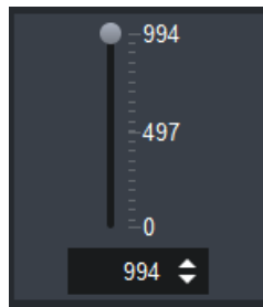
Figure 28 - WIDGET_SLIDER_VERTICAL hint
